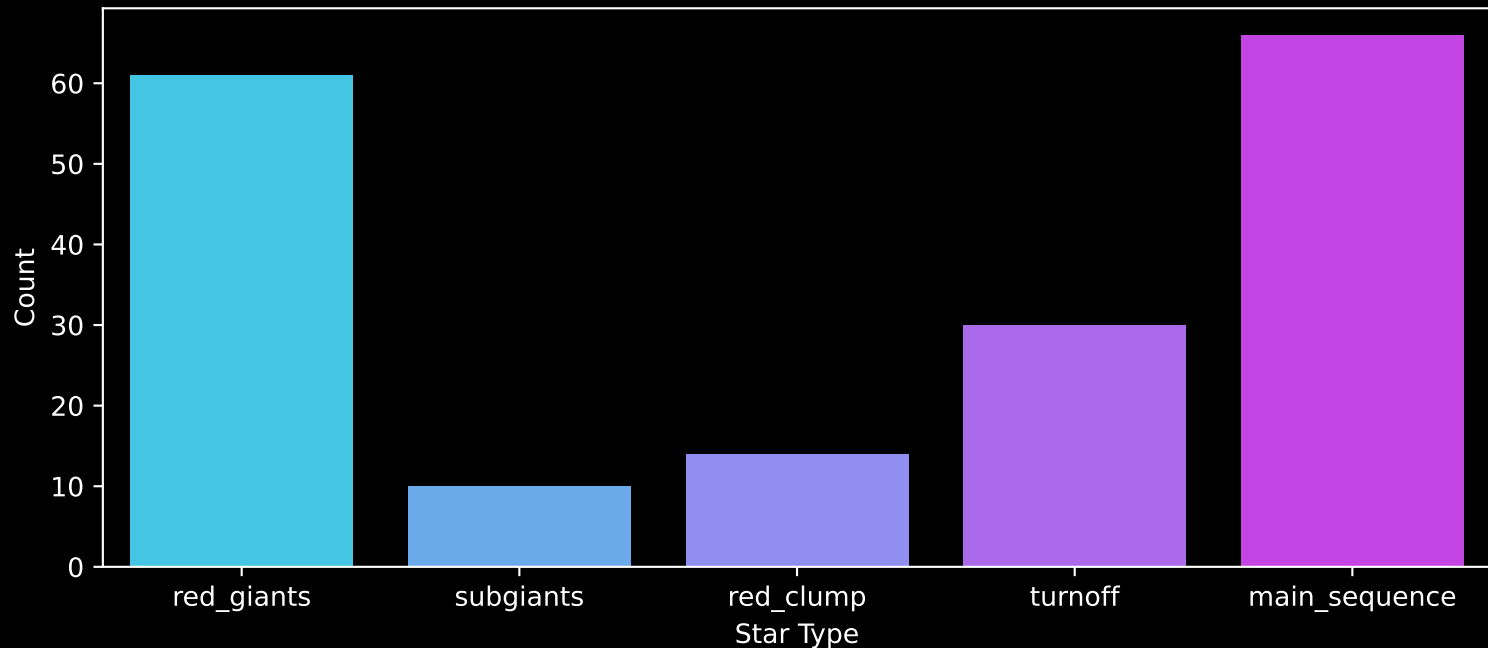
APOGEE DR17 Field: [CVZTILE_088+35_btx] Count plot of Star Type
