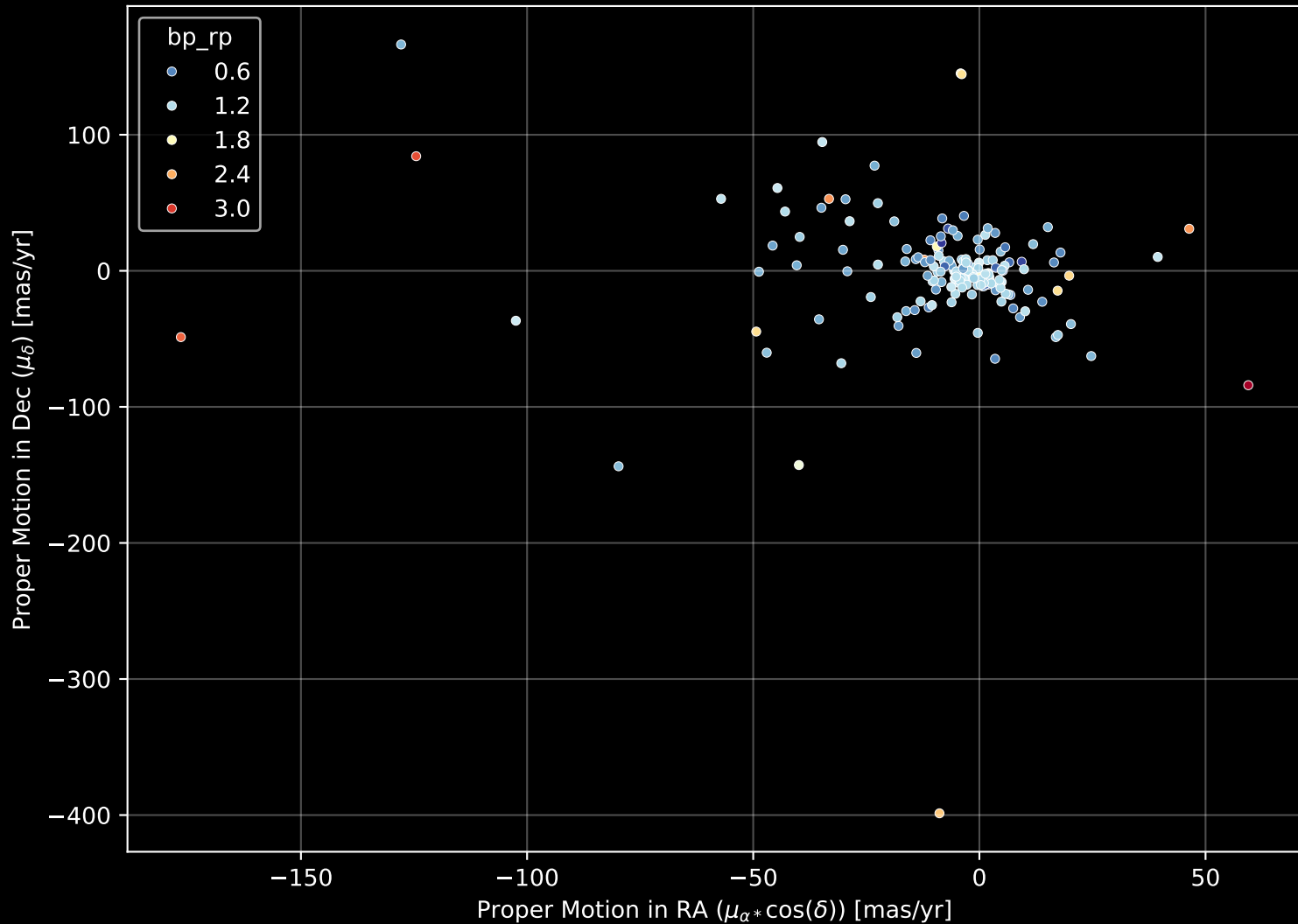
APOGEE DR17 Field: [CVZTILE_088+35_btx] Proper Motion Diagram (n= 181)
