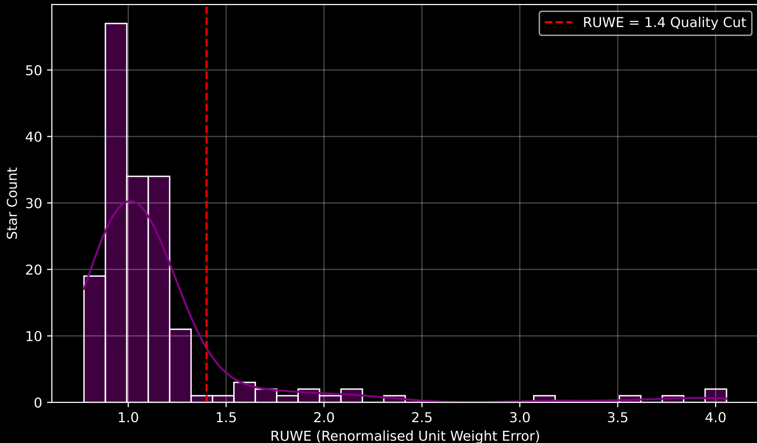
GAPOGEE DR17 Field [CVZTILE_088+35_btx] RUWE Distribution (n= 174)
