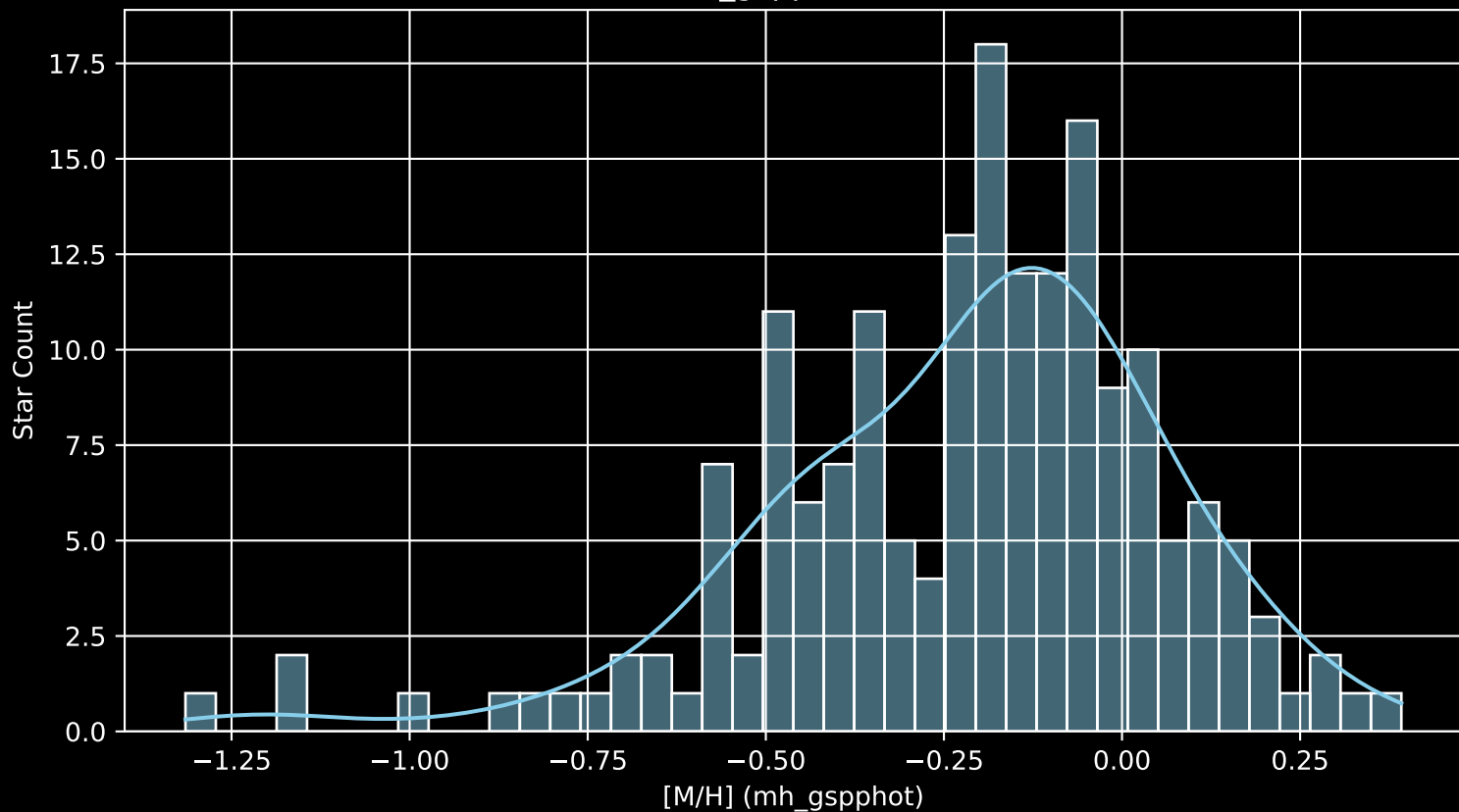
APOGEE DR17 Field: [CVZTILE_088+35_btx [M/H] (mh_gspphot) (n= 180)
